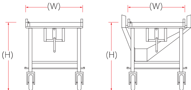
Front View Model : MAC -1 (Without downdraft)
